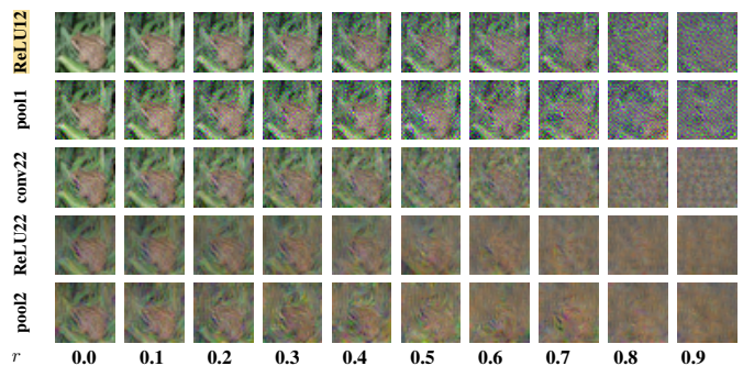
Fig. 12: Dropout as a defense against attacks at different layers on CIFAR10 dataset. Rows from top to bottom: ReLU12, pool1, conv22, ReLU22, pool2.
