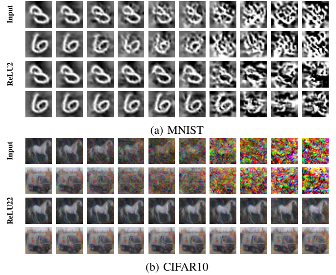
Fig. 7: Examples of adding Laplacian noise to defend against white-box attack on MNIST (ReLU2) and CIFAR10 (ReLU22). b is the standard deviation of the Laplacian noise.
