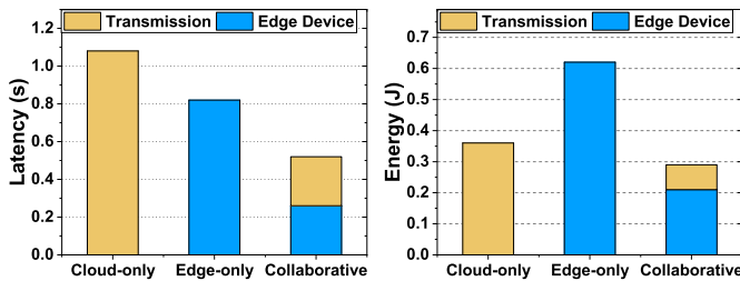
Fig. 2: Breakdown of inference latency (left) and energy consumption (right) in edge-cloud systems. Data are from [8].
